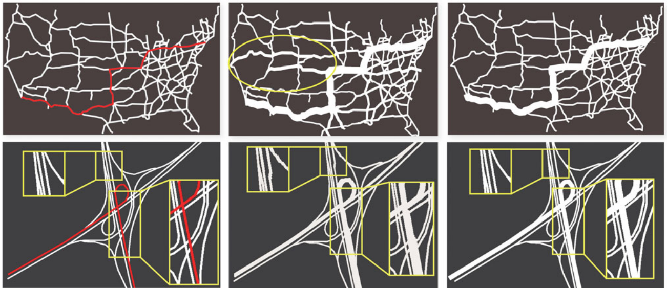
Fig. 4. Technique comparison with US highway maps and a complex road junction. The focus routes are highlighted in red in the left two figures, the middle two figures are the results created by the seam carving based method, and the right two figures are the ones created by our route-zooming method.
