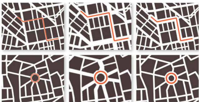
Fig. 5. Comparison of the route-zooming algorithm with the seam carving based method for broadening a focus route highlighted in red.
