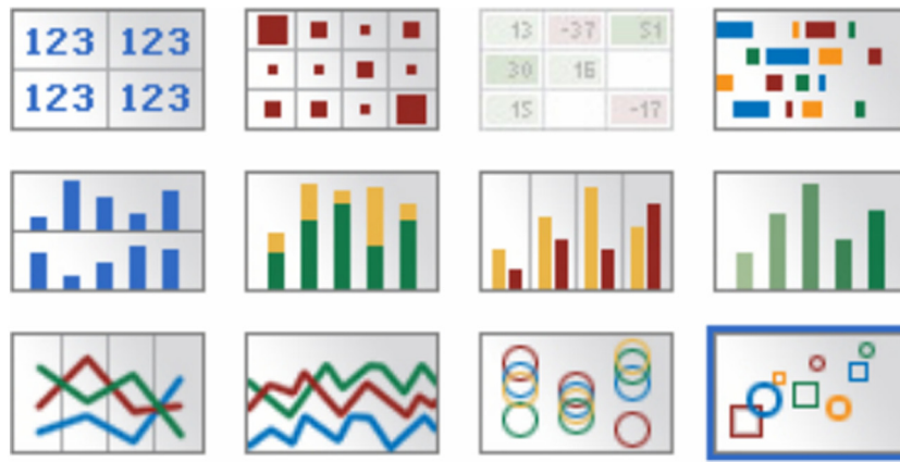
Fig. 12. The Ranking of alternative visualizations of Show Me (Mackinlay et al., 2007). Users can iteratively make a choice of visualization recommendations.
